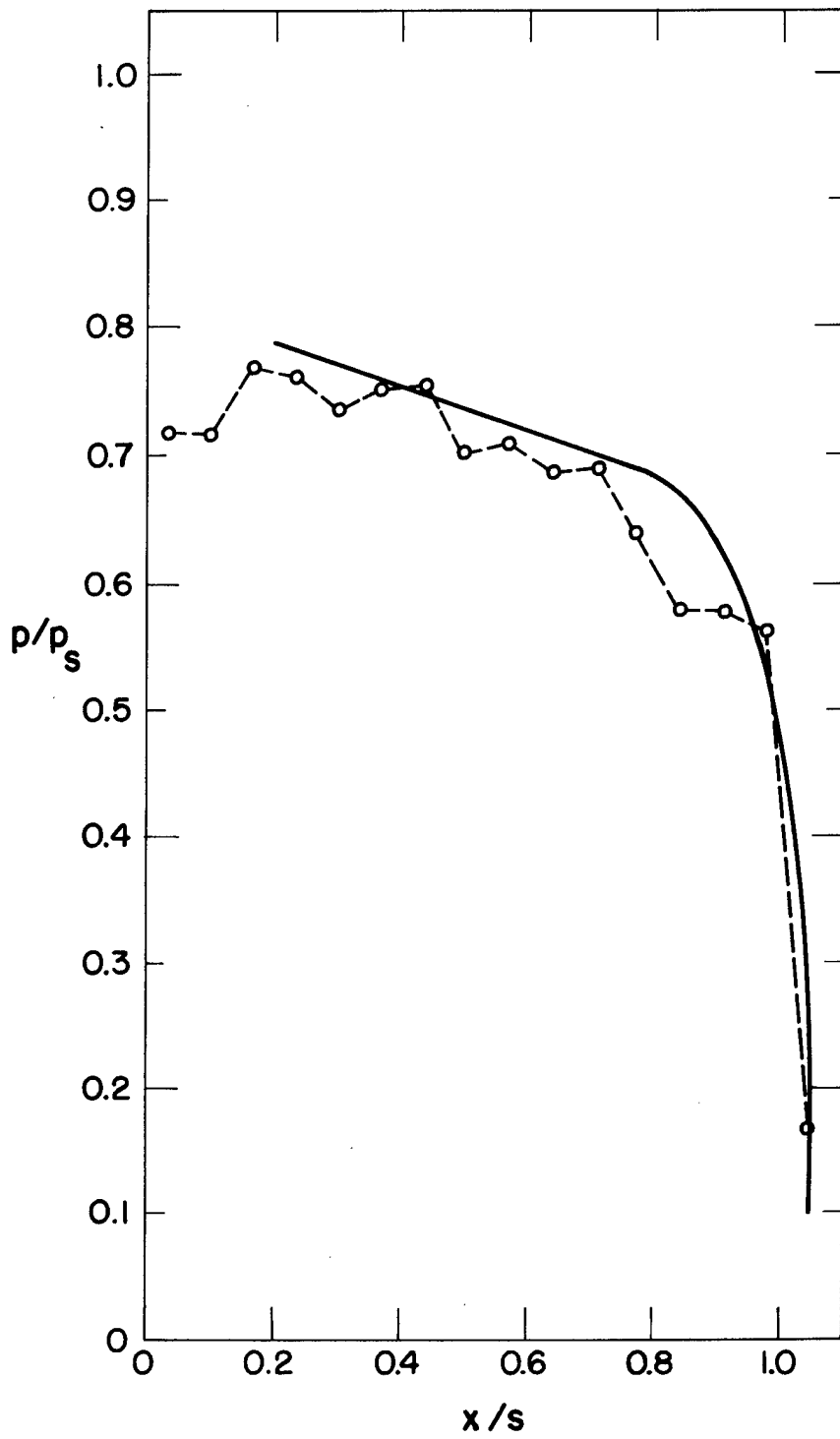
Figure 8. Obstacle pressures, 75° cone. Mach 1.58
